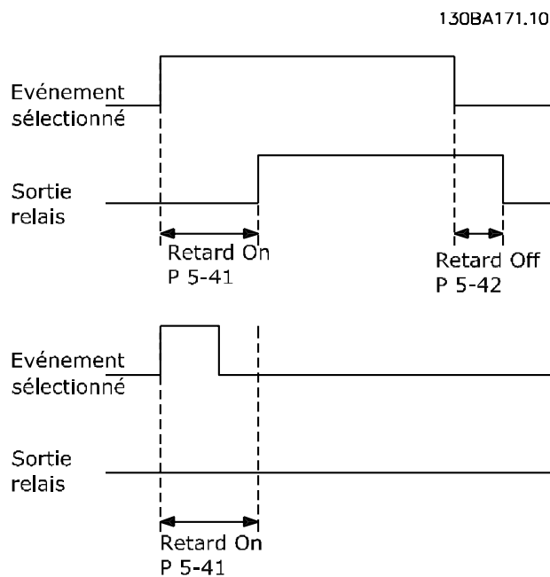
Illustration 3.25 Relais, retard ON
