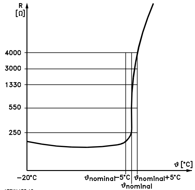
175HA183.10 Illustration 3.11 Profil PTC
