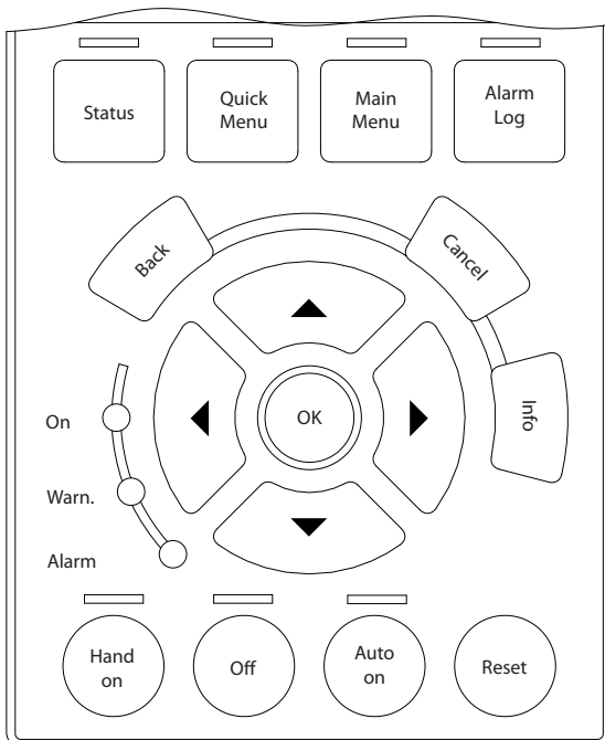
Illustration 2.18 LCP
