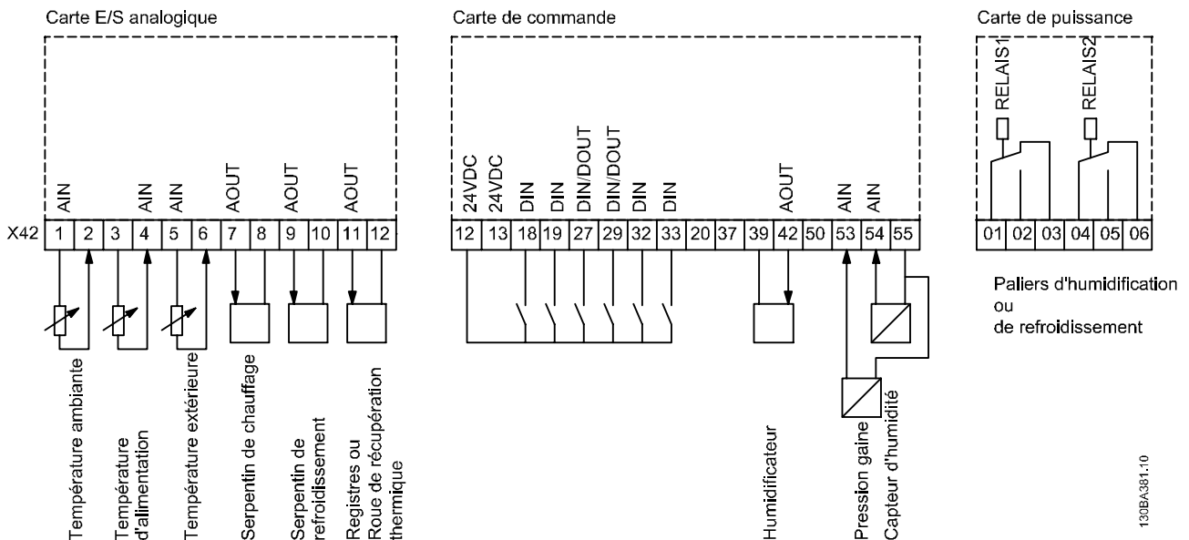
Illustration 3.83 Option E/S ana. MCB 109
