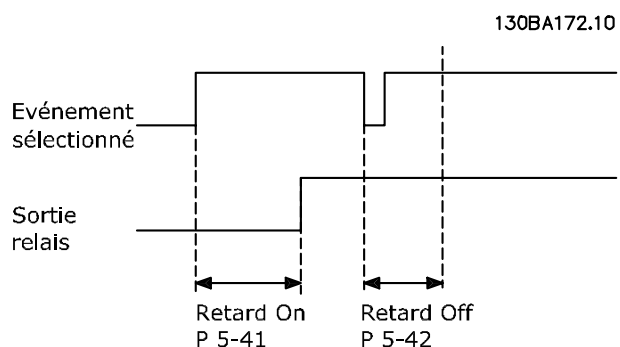
Illustration 3.26 Relais, retard OFF
