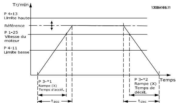
Illustration 3.20 Rampe 1
