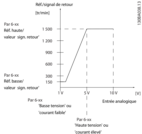
Illustration 3.29 Conditions zéro signal
