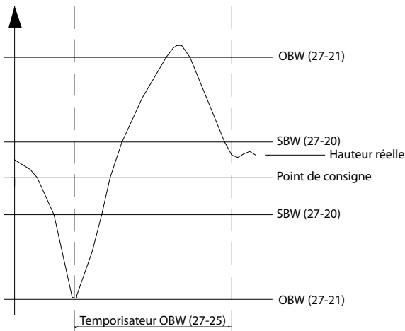
Illustration 3.74 Tps OBW
