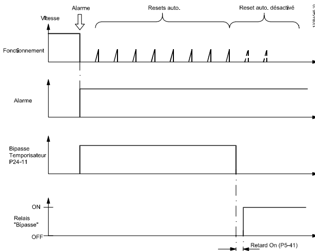
Illustration 3.66 Bypass variateur
