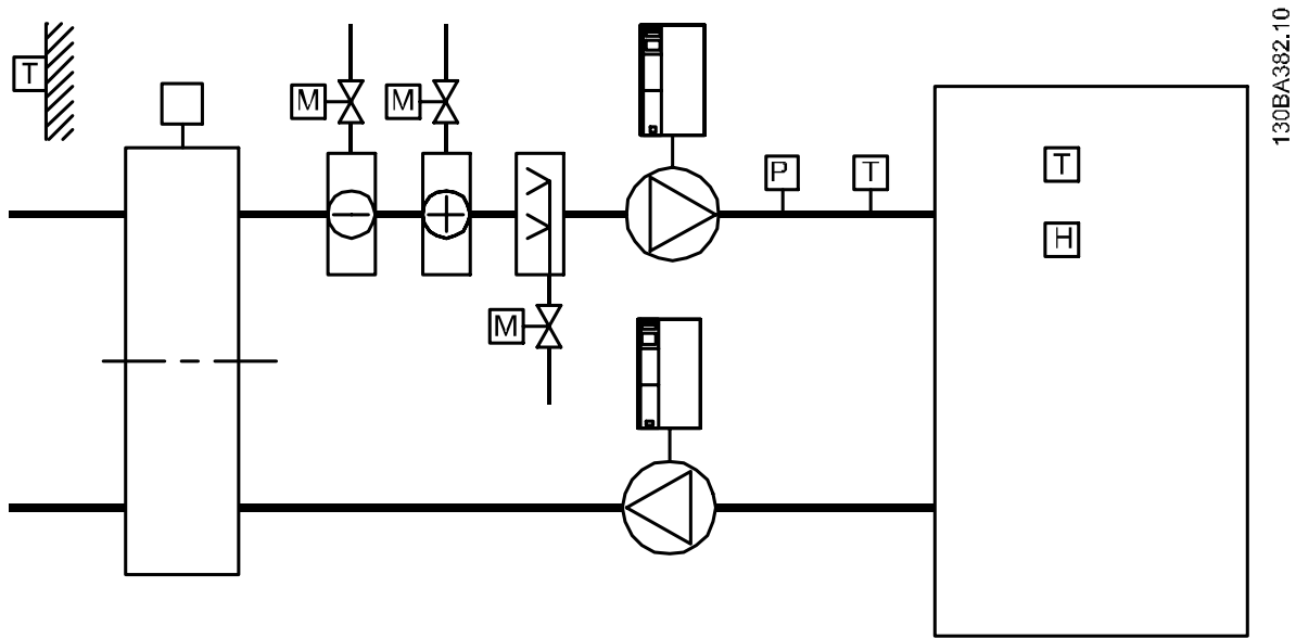
Illustration 3.82 Option E/S ana. MCB 109
