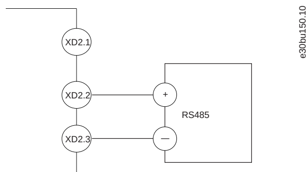
Illustration 57: Raccordement du câblage RS485
