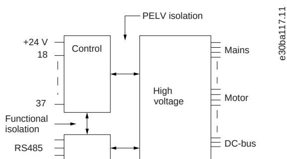
Illustration 71: Isolation PELV
